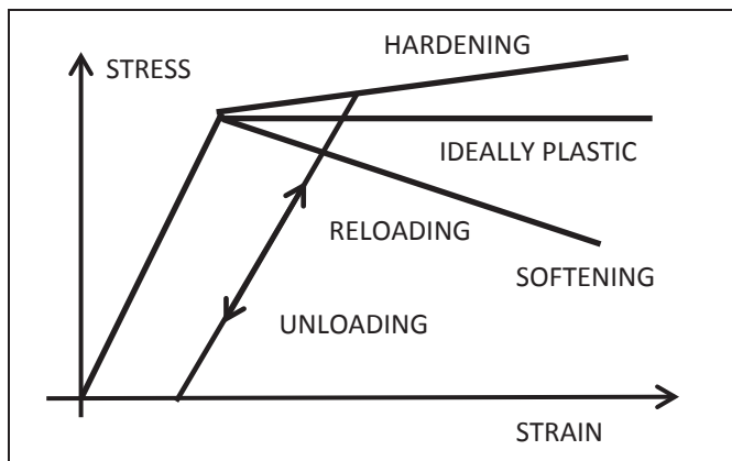
Figure 1. Idealized uniaxial stress-strain plots
