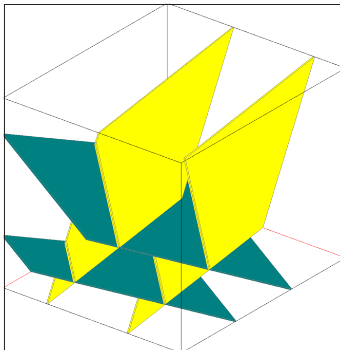
Figure 2. Schematic illustration of the two joint sets used in computing equivalent properties
