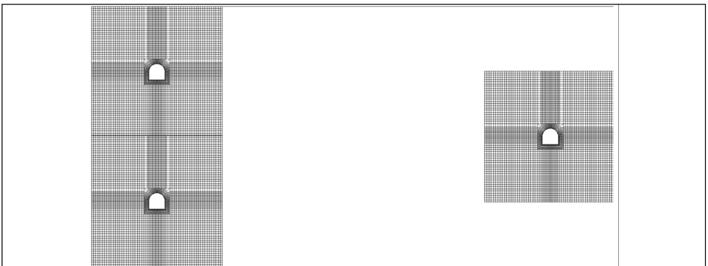
Figure 7. A cross-section of a spiral ramp with a design grade of 15 percent. The ramp is circular so sections are at 0, 180 and 360 deg are shown. The section is 11x11 ft (3.4x3.4 m). The spiral radius is 11.25 times opening width or 123.74 ft (37.7 m)
