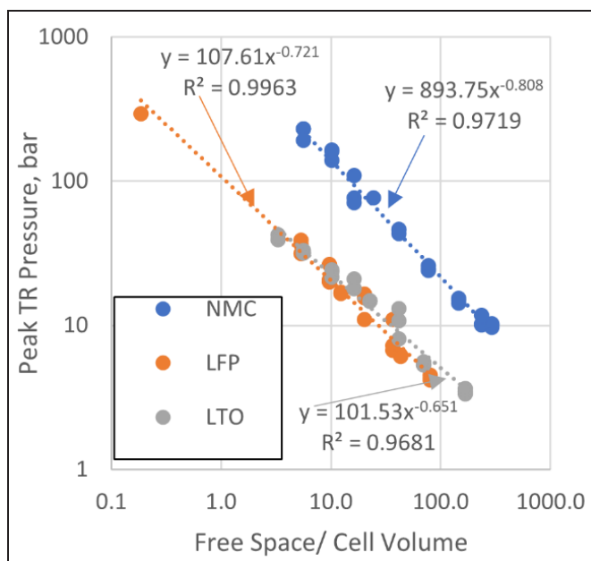
Figure 15. Comparison of peak thermal runaway pressures from LTO, LFP [14], NMC [14] cells
