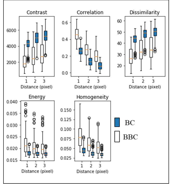
Figure 4. Box plots of various GLCM features with different distance values
