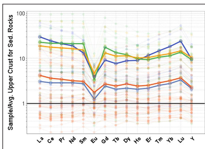
Figure 8. Average Upper Crust for Sedimentary Rocks-normalized spider diagram (Taylor and McLennan, 1981) of heavy mineral sandstones showing highly elevated REE, slight heavy REE enrichment, and prominent negative Eu anomalies. Legend in Figure 7
