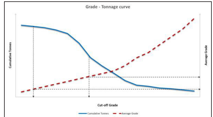
Figure 4. Example of Graphical of grade- tonnage curve
