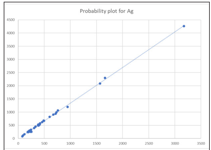
Figure 5. Probability plot for Ag element
