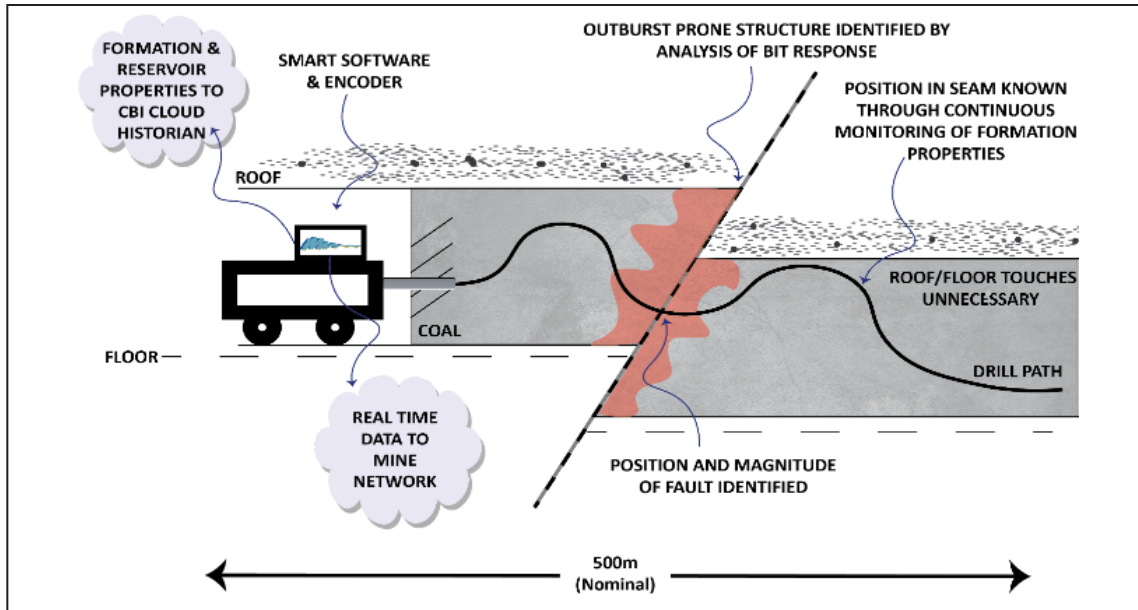
Figure 1. Schematic showing how the Yabby GeoSensing system provides information to improve geological models
