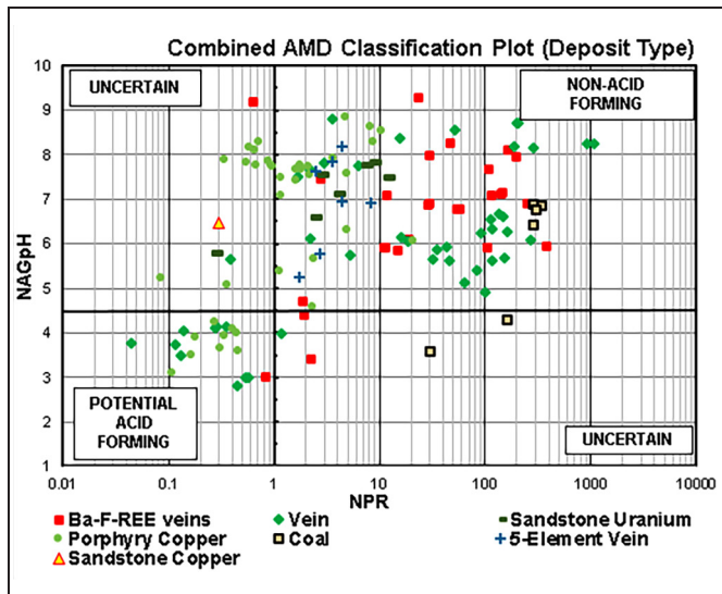
Figure 10. Acid Rock Drainage (ARD) plot of waste rock pile at mines examined during the NMBGMR mine wastes project
