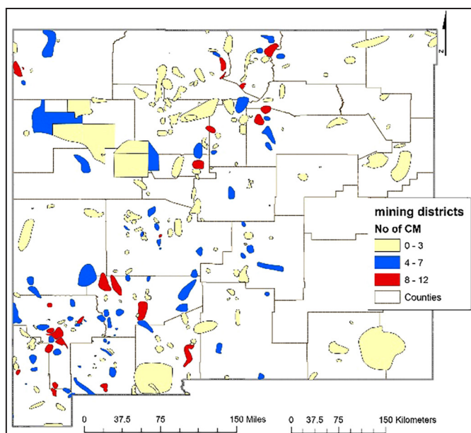
Figure 1. Map of mining districts in New Mexico that have critical minerals. Coal fields are not shown. Other areas in New Mexico, such as high-magnesium dolomites, lithium-bearing playas, and coal fields, are not found in specific mining districts and also have potential for critical minerals (CM)
