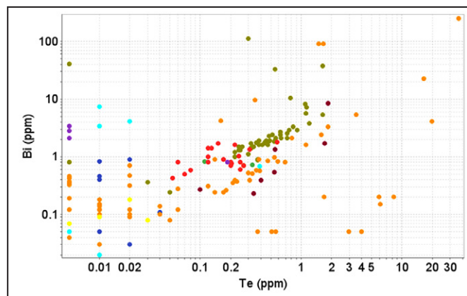
Figure 9. Bi versus Te for samples from mining districts in New Mexico. See Table 1 for summary of districts and different deposit types sampled, and Figure 3 for locations. Legend is in Figure 7
