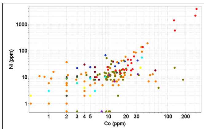
Figure 8. Ni versus Co for samples from mining districts in New Mexico. See Table 1 for summary of districts sampled and different deposit types, and Figure 3 for locations. Legend is in Figure 7
