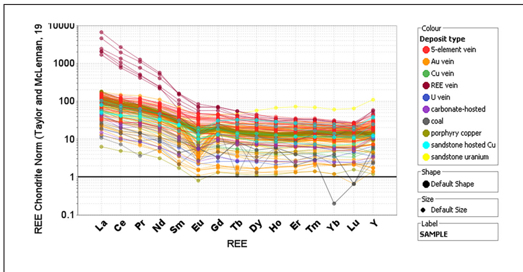
Figure 7. Chondrite-normalized (Taylor and McLennan, 1985) rare earth elements (REE) for samples from mining districts and different deposit types in New Mexico. See Table 1 for summary of districts sampled and Figure 3 for locations
