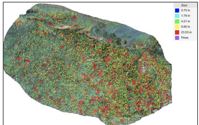
Figure 6. 3D fragmentation model built using BlastMetrix
