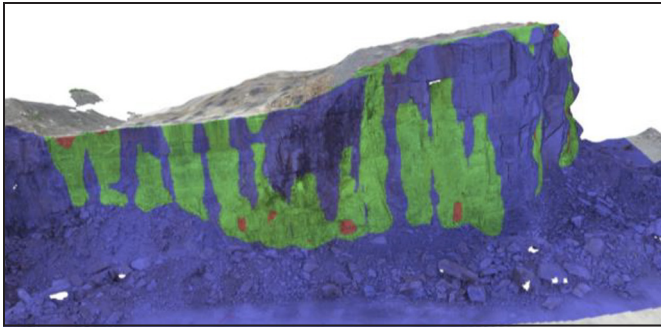
Figure 4. Minimum burden for the entire highwall face (optimized) looking towards the east. Legend. Green-10 feet (3 meters), Red – 9 feet (2.7 meters), and Blue – 11 feet (3.3 meters)
