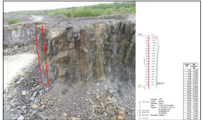
Figure 2. Minimum burden for the highwall face looking towards the north
