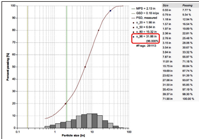
Figure 7. Muck pile particle distribution curve generated for P80; highlighted the percentage of passing the material through the primary stage crusher
