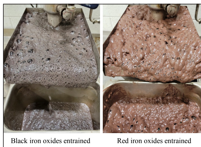
Figure 4. Ultrafine black and red iron oxides entrained during benchtop mechanical cell flotation
