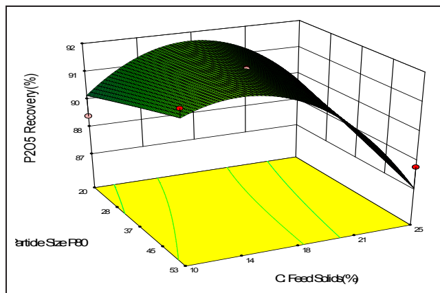
Figure 12. Floated concentrate P 2 O 5 recovery vs feed particle size and feed slurry solids content
