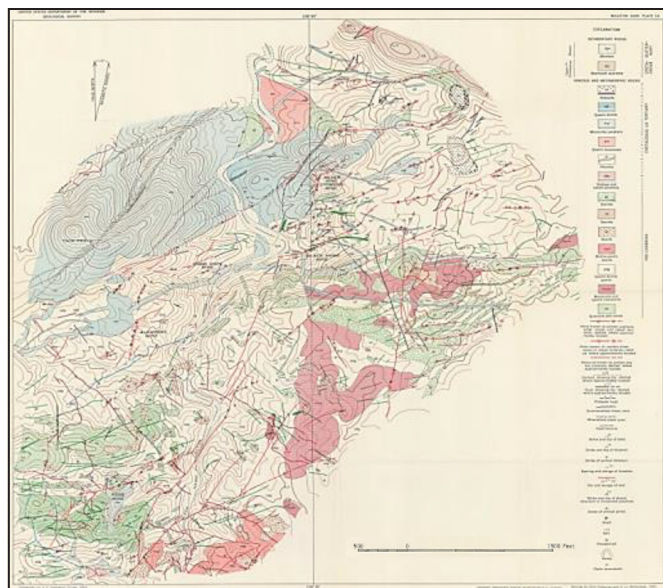
Figure 3. Geologic map of the Black Hawk mining district, Grant County, New Mexico. From (Gillerman & Whitebread, 1953)
