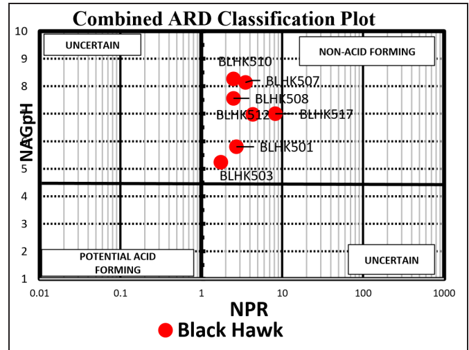
Figure 10. Acid Rock Drainaige (ARD) graph of Black Hawk mine waste samples
