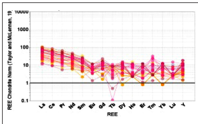
Figure 4. Chondrite normalized patterns of Coal
