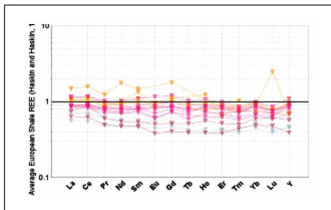
Figure 7. Clinker normalized to Average European Shale
