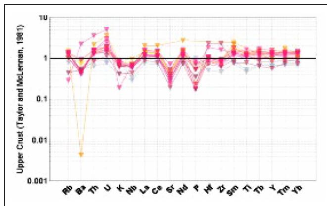
Figure 6. Clinker normalized to Average Upper Crust for Sedimentary Rocks
