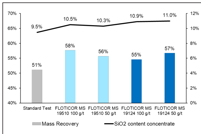
Figure 5. Tests results using agglomerating agents as additives
