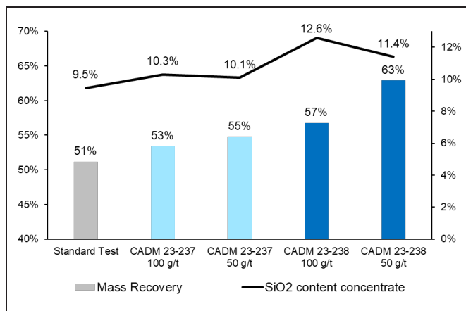
Figure 6. Tests results using rheology modifiers as additives
