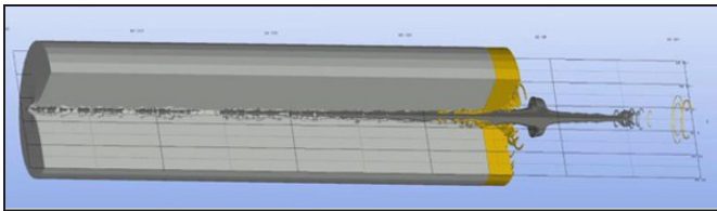
Figure 3. Shape charge detonation computer model
